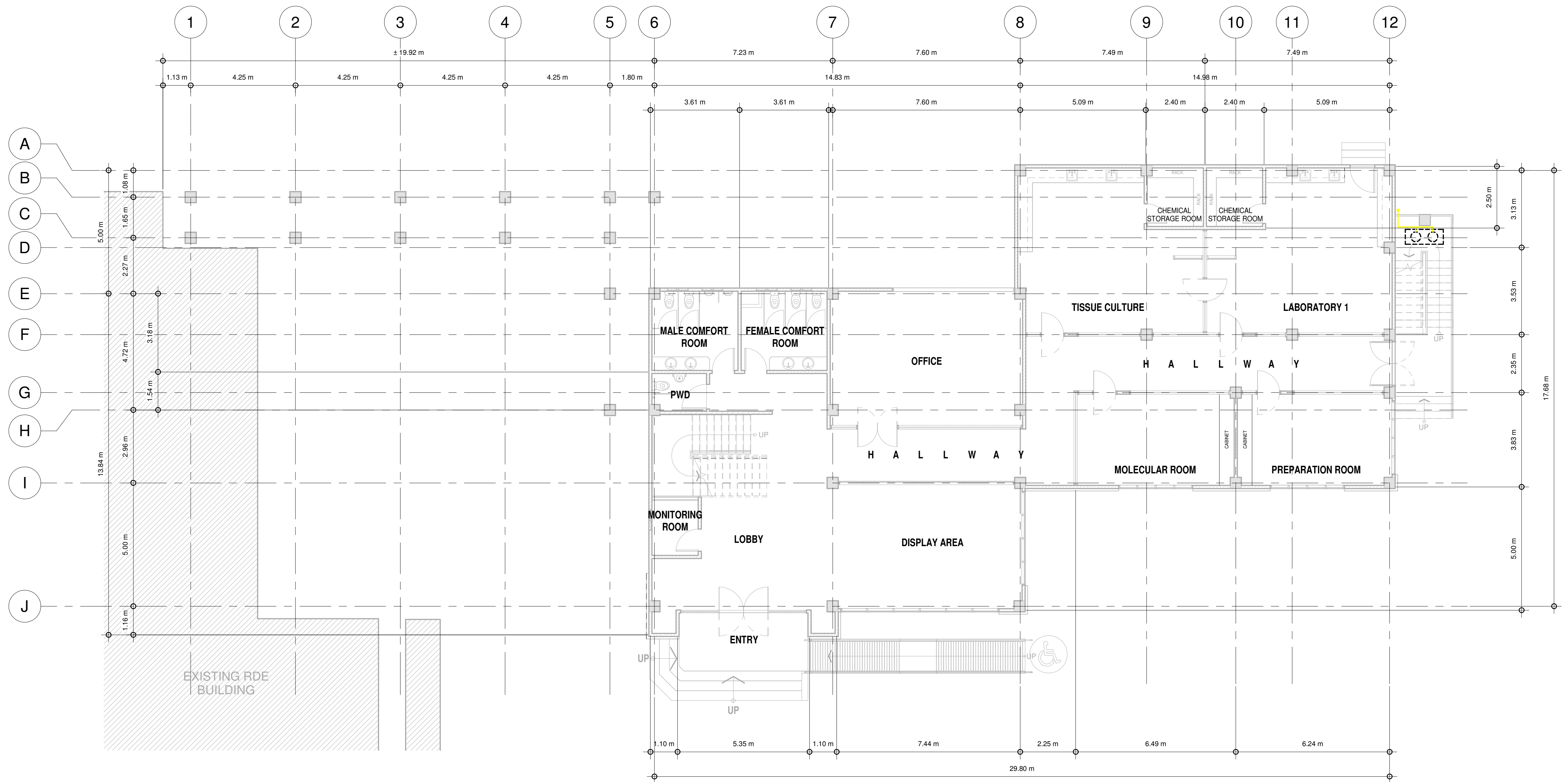
1 GROUND FLOOR GAS LINE LAYOUT PLAN 1 : 100 meters
